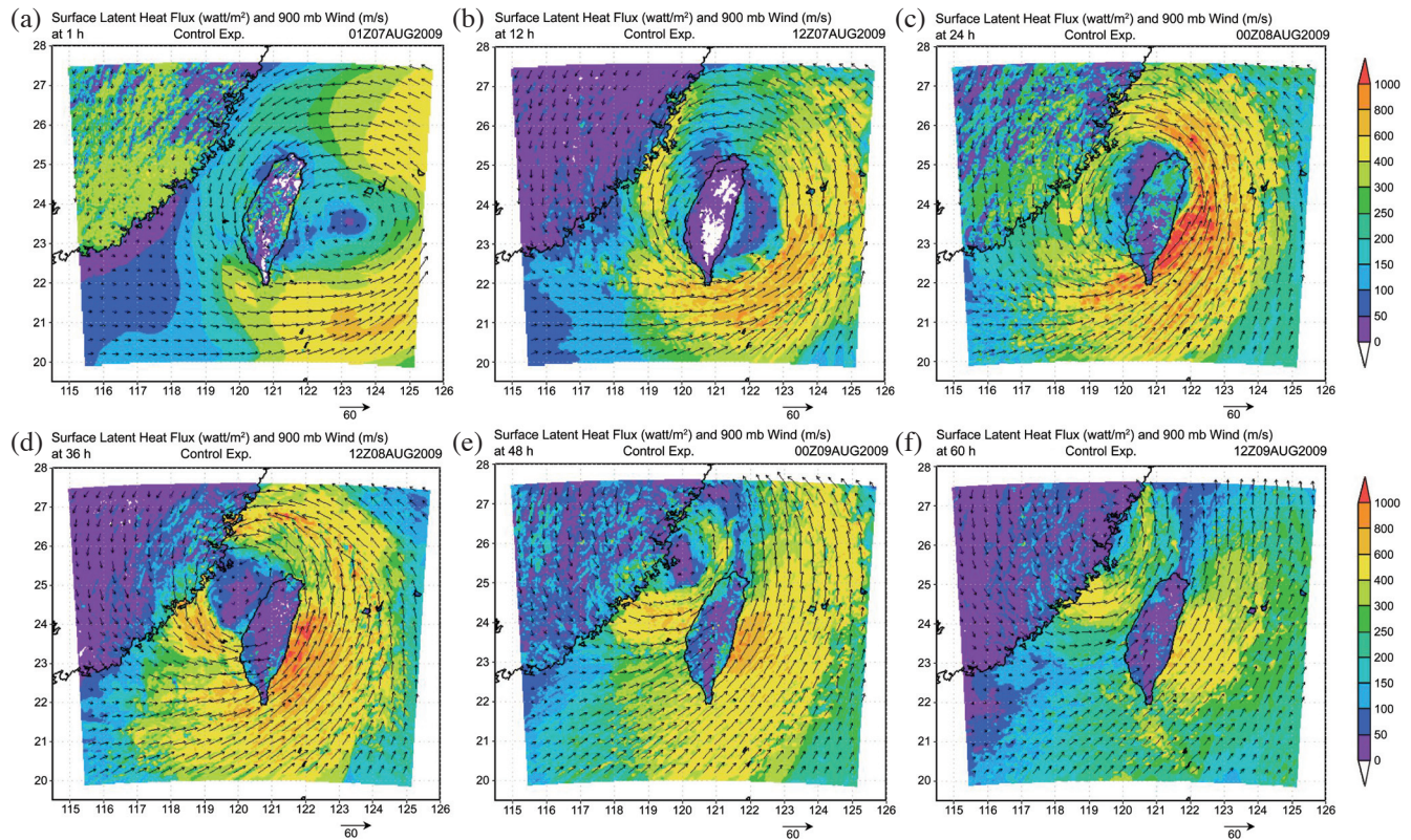
Fig. 6. Simulated surface latent heat flux ( \text{W m}^{-2} , shaded) and 900 hPa wind ( \text{m s}^{-1} , vectors) at (a) 1, (b) 12, (c) 24, (d) 36, (e) 48 and (f) 60 hours of integration for the control run.
