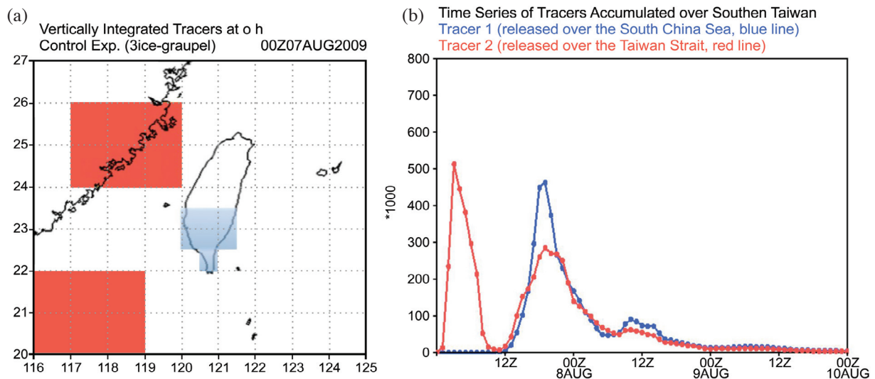
Fig. 7. (a) Geographic locations of the initial inert tracer and (b) temporal- and domain-integrated tracer for the region of Taiwan located south of 23^{\circ}\text{N} where the heavy rain occurred.
