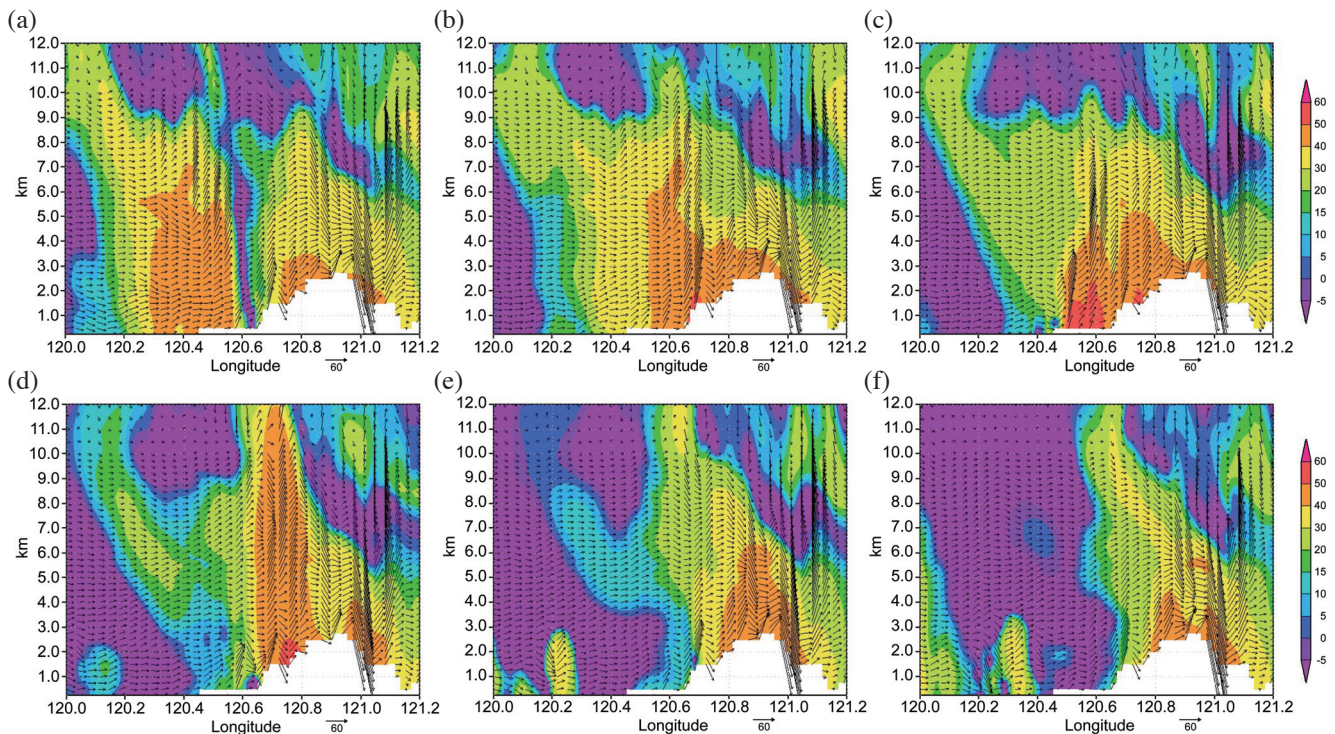
Fig. 9. Simulated radar reflectivity (dBZ, shaded) and wind ( \text{m s}^{-1} , vectors) at 23.0°N at (a) 1550 UTC, (b) 1600 UTC, (c) 1610 UTC, (d) 1620 UTC, (e) 1630 UTC and (f) 1640 UTC on 8 August 2009.
