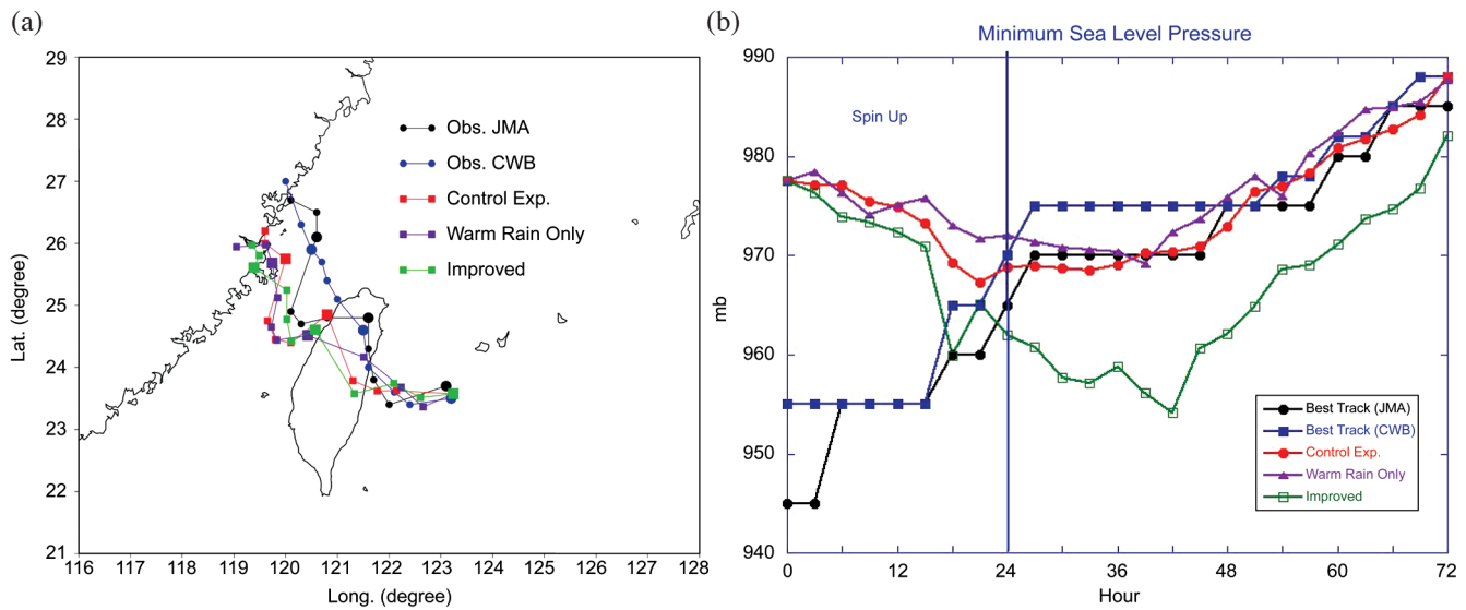
Fig. 11. Same as Fig. 2 except for the simulations with improved microphysics and warm rain only.
