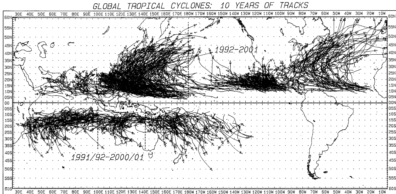
Figure 1 Tracks of tropical cyclones with wind speeds of at least 17 \text{ ms}^{-1} for the period 1992–2001. Courtesy of Dr. Charles Neumann (Neumann 1993).
